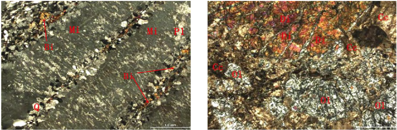
图4 JC14 薄片正交偏光2.5×,花岗质混合片麻岩(左),JC57-1薄片正交偏光2.5×,大理岩(右) Fig.4 JC14 slice perpendicular-polarized light 2.5×,granitic migmatitic gneiss(left), JC57-1 slice perpendicular-polarized light 2.5×,marble (right)
